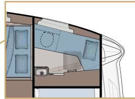
Option for an Additional Forepeak Crew Cabin
