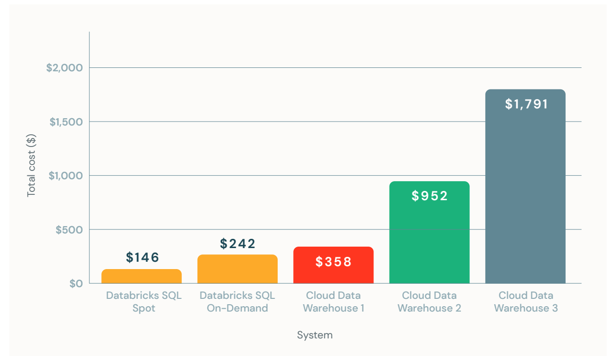
100TB TPC-DS price/performance benchmark (lower is better).
