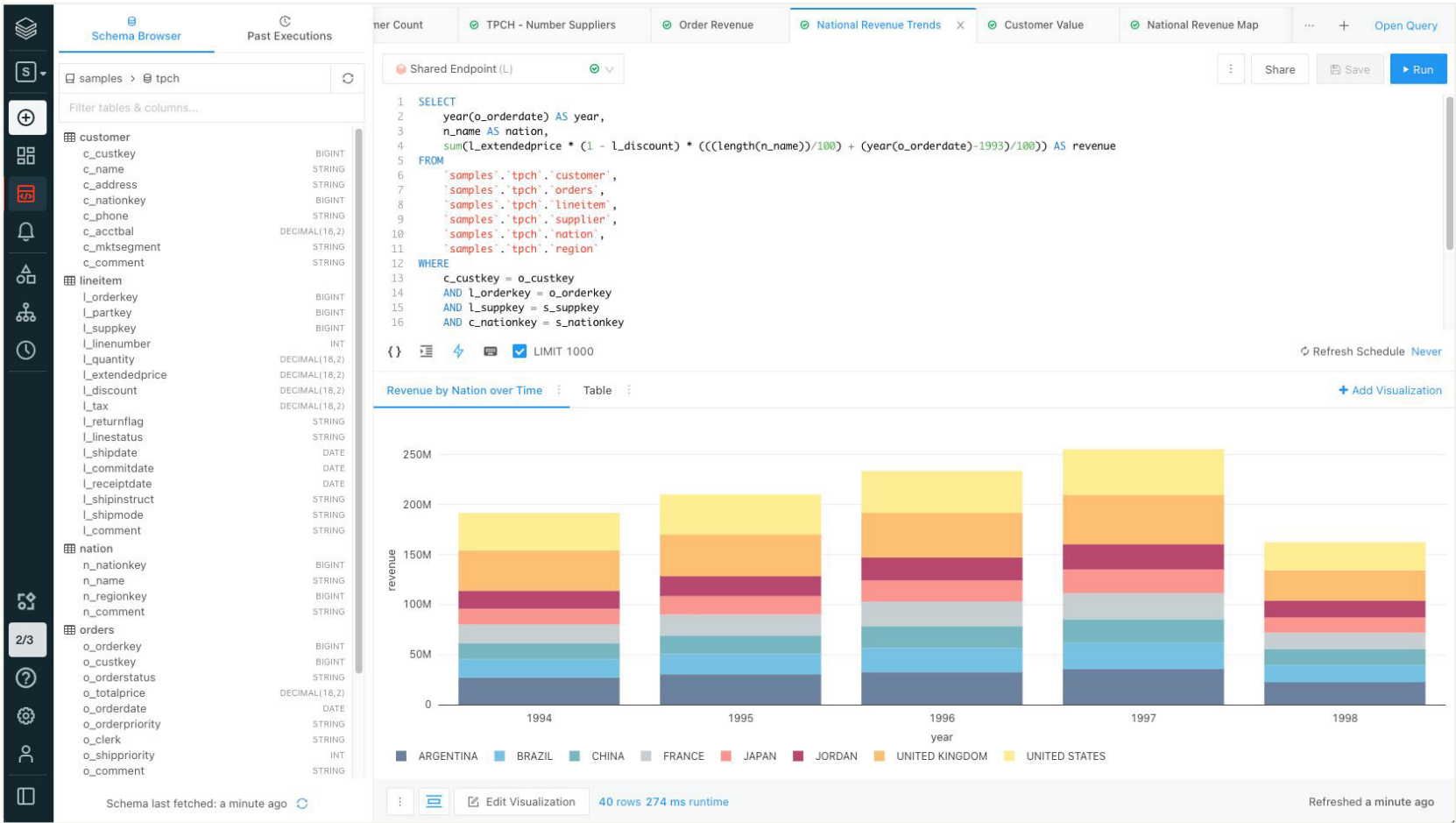
The built-in SQL query editor allows you to quickly explore available databases, query and visualize results.
