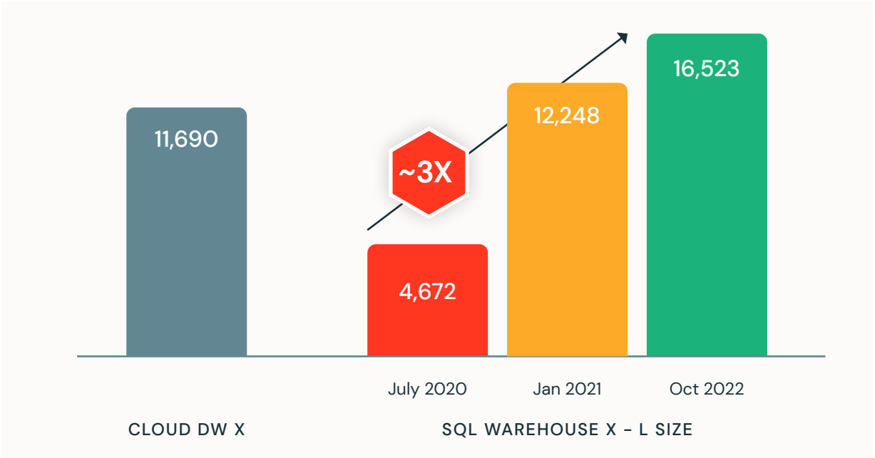
10GB TPC-DS queries/hr at 32 concurrent streams (higher is better).
