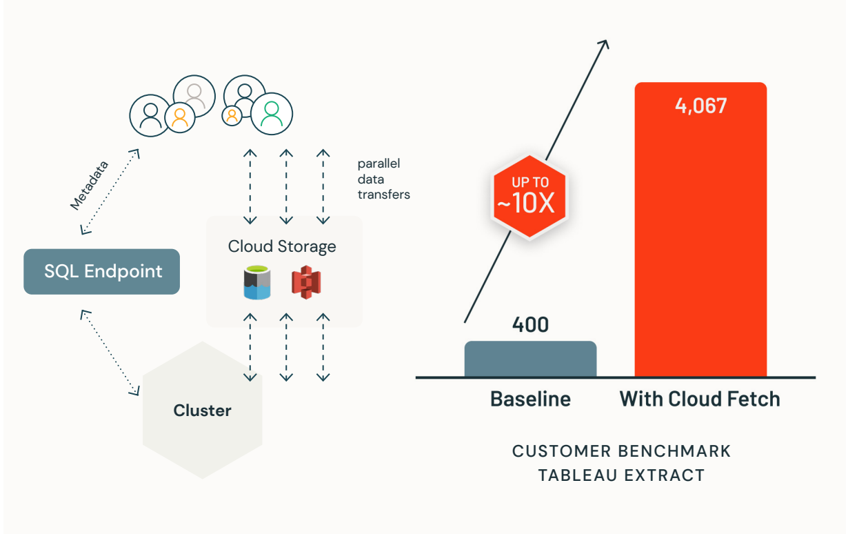
Cloud Fetch enables faster, higher-bandwidth connectivity to and from your BI tools.
