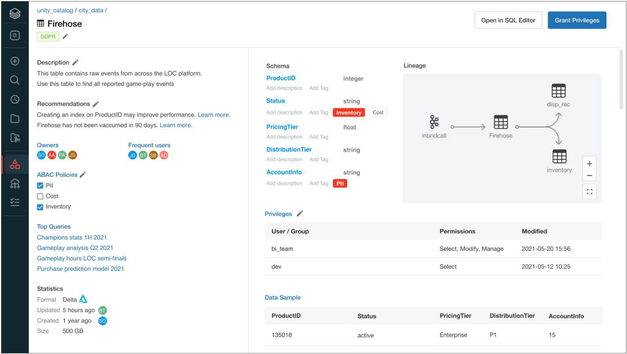
The Unity Catalog makes it easy for data stewards to discover, manage and secure data access to meet compliance and privacy needs on the lakehouse.
