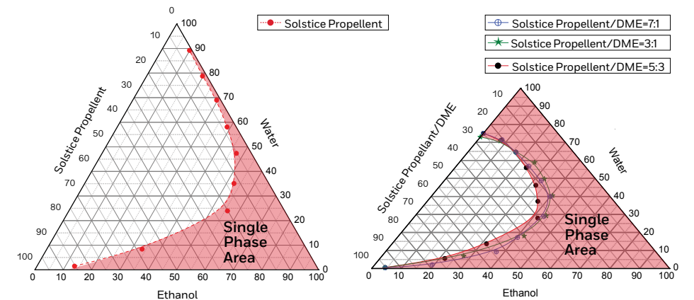
Figure 3. Single-phase area of three ingredients Figure 4. Single-phase area of three components
