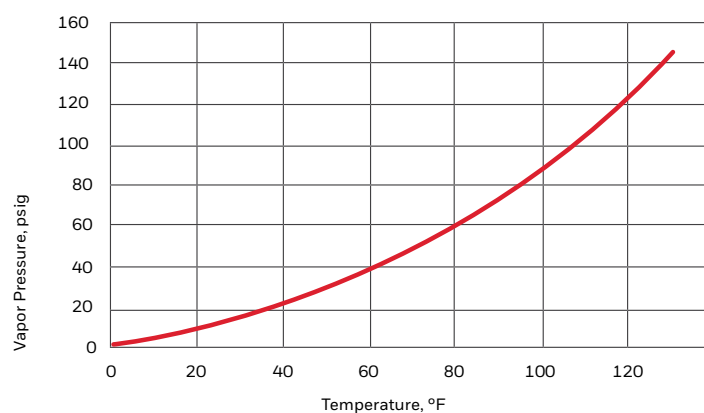
Figure 1. Vapor Pressure vs. Temperature (English Units)
