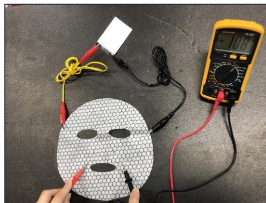
Conductivity Test - Measured current: 1.08 \mu A
